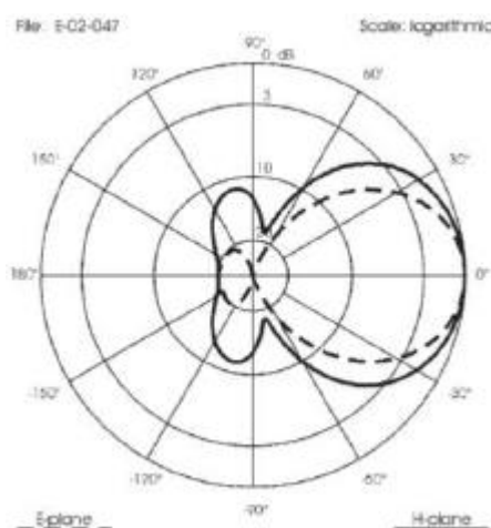
Radiation pattern
